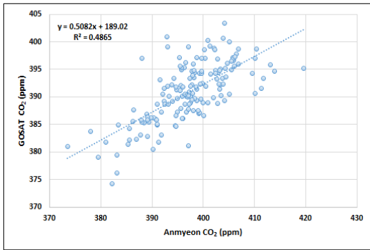
Figure 4. Correlation between GOSAT and Ground measurement
